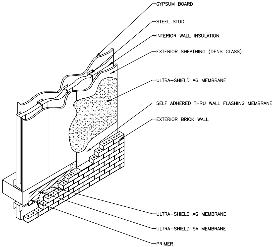
○ AIR BARRIER WARM CLIMATE W/DENS GLAS ARCH. REF.:
